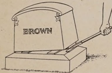
Always Place Wood Between Stone and Crowbar.
